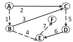
Figure 1: Graph G
