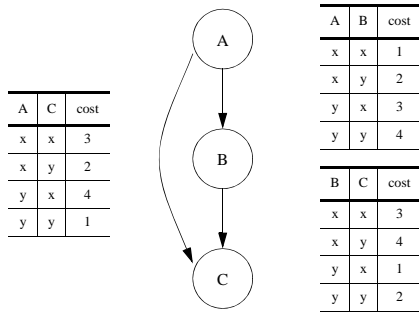
Figure 1: Example DCOP
