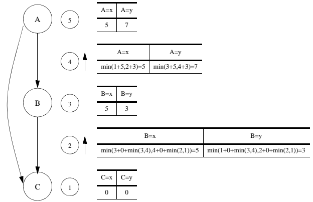
Figure 3: DP2 Example
