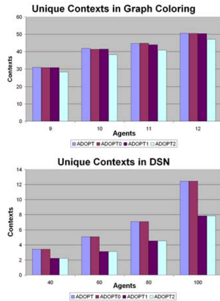
Figure 9: Unique Contexts
