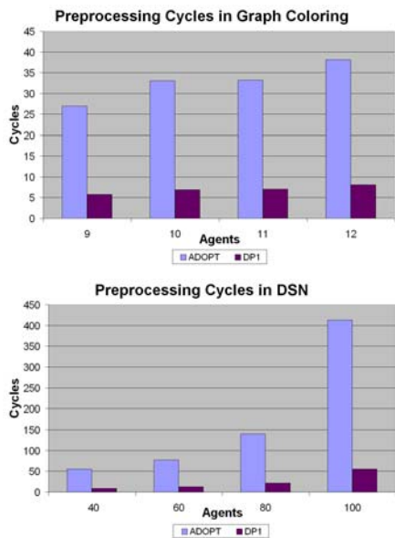
Figure 6: Preprocessing Cycles
