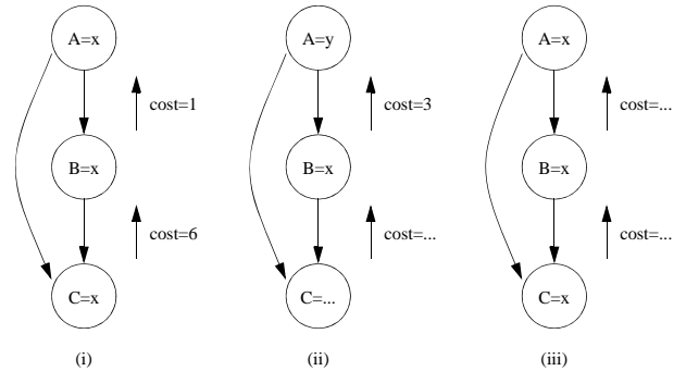
Figure 2: Possible Execution Trace of ADOPT
