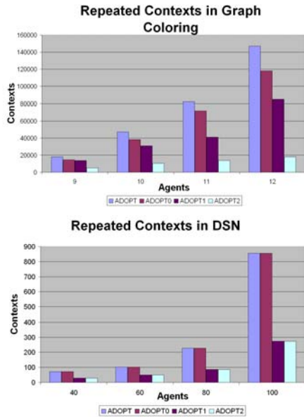
Figure 8: Repeated Contexts
