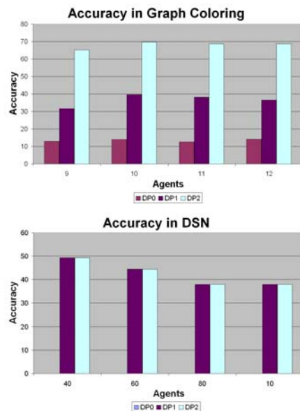
Figure 7: Accuracy
